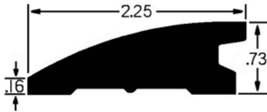
3/4" Reducer (H34BR)
