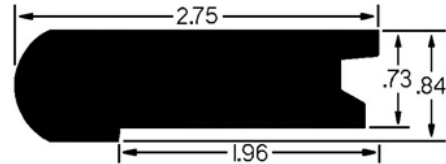
3/4" Nosing (H34BN)
