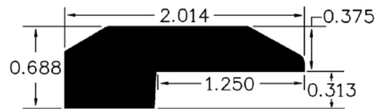
EndCap/Threshold (HBATH)
